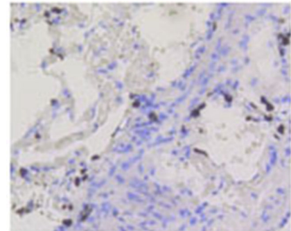
Fig. 2. Immunohistochemical analysis of paraffin-embedded human lung tissue using anti-BDNF antibody. Counter stained with hematoxylin.
