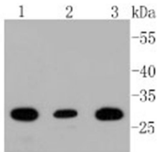
Fig. 1. Western blot analysis of BDNF on different lysates using anti-BDNF antibody at 1/1,000 dilution. Positive control: Lane 1: SHG-44; Lane 2: A172; Lane 3: Mouse brain
